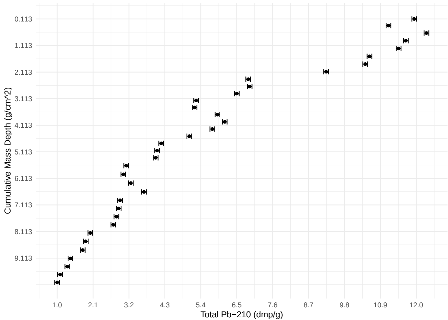
Total Pb-210 vs Cumulative Mass Depth
